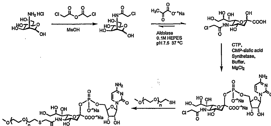
Scheme 5
